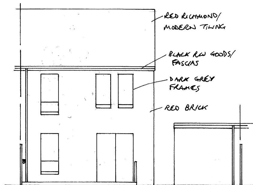
EXISTING REAR 1:100
