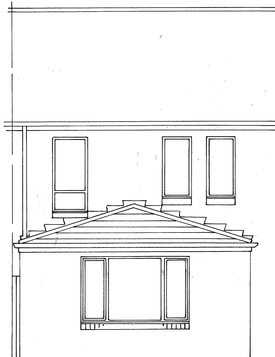
PROPOSED REAR 1:50
